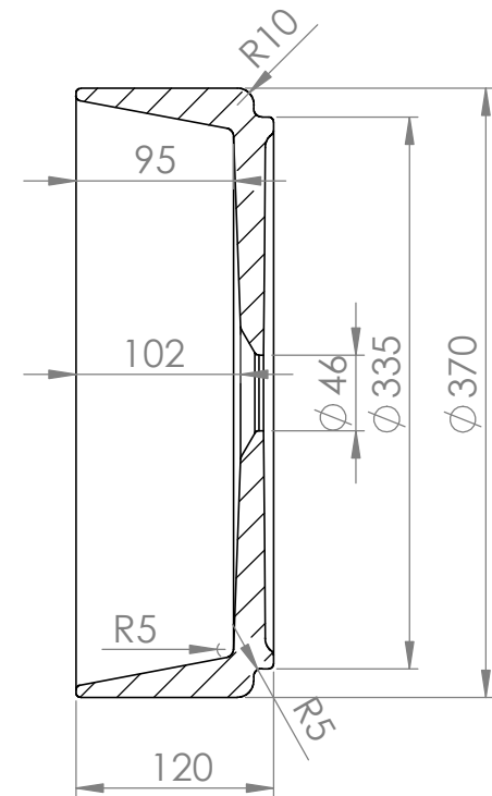
SECTION C-C'
